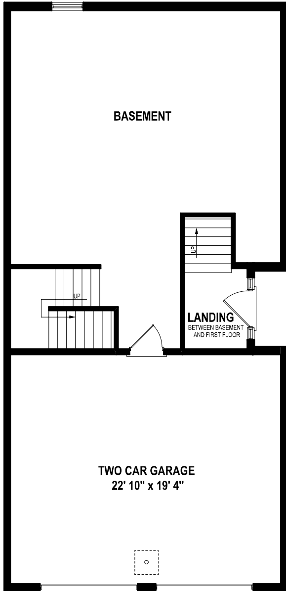
FOUNDATION PLAN
