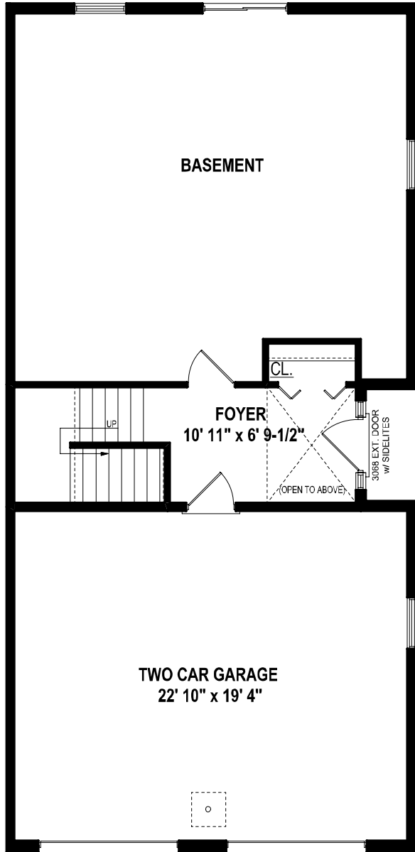
FOUNDATION PLAN
